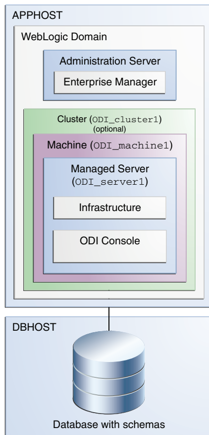
Figure C-1 Secondary Installation Topology including the ODI Console
