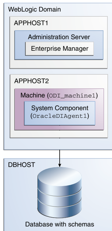
Figure 1–3 Standard Installation Topology for the Standalone Colocated Agent
